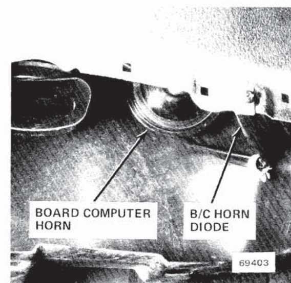
Figure 5 - Under LH Side of Front Bumper (Splash Guard Pulled Down)
