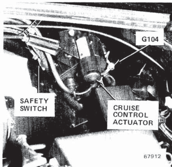
Figure 1 - Forward of LH Front Wheel Well
