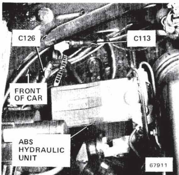
Figure 2 - LH Front of Engine Compartment (Cover Removed)
